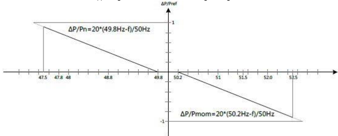
Figure 6 MODEL SOFAR 125KTLX-G4-A P(f)-diagram
