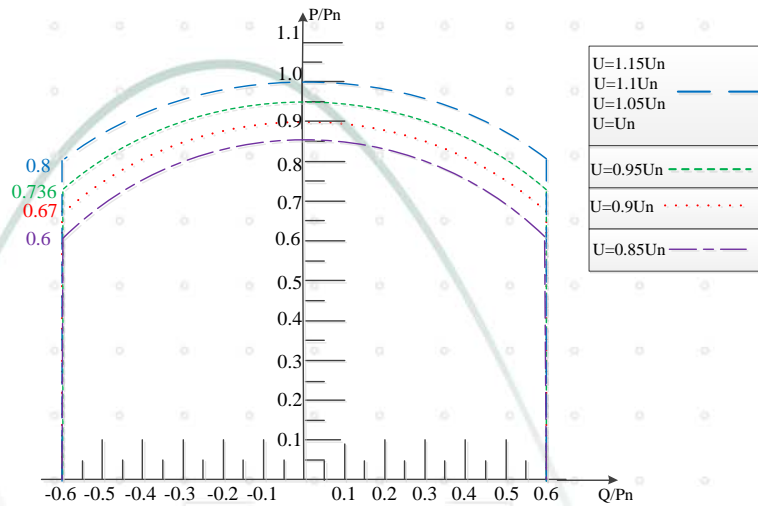
Figure 4 a. Voltage-dependent PQ diagram for MODEL SOFAR 125KTLX-G4-A and SOFAR 100KTLX-G4
