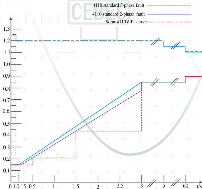
Figure 5 FRT limit curve for SOFAR 125KTLX-G4-A
