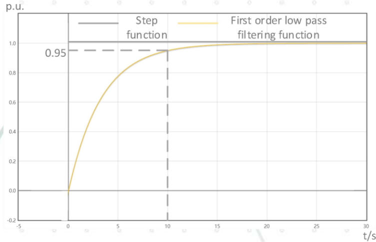
Figure 7 MODEL SOFAR 125KTLX-G4-A reactive power control feature
