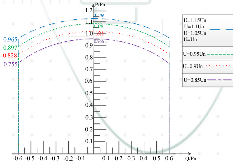
Figure 4. b. Voltage-dependent PQ diagram for MODEL SOFAR 125KTLX-G4
