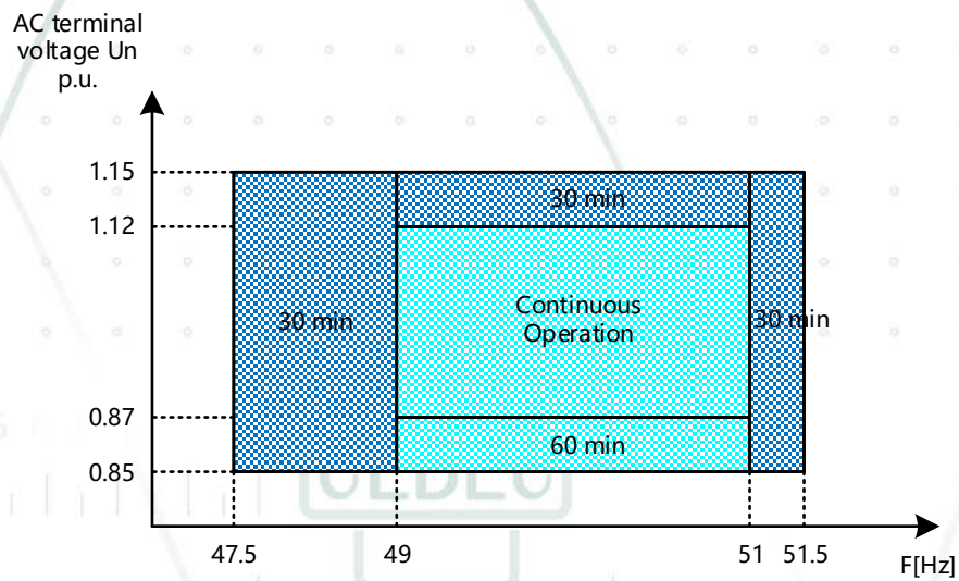
Figure 3 Quasi-stationary operation range for MODEL SOFAR 125KTLX-G4-A
