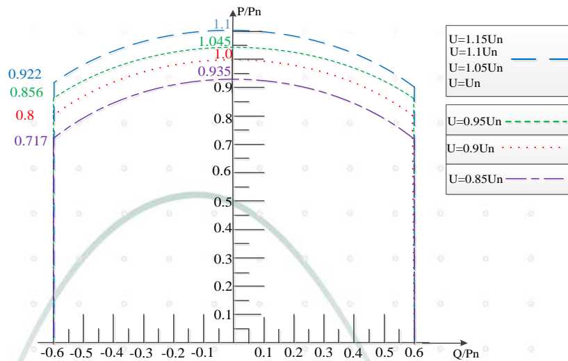
Figure 4.c Voltage-dependent PQ diagram for MODEL SOFAR 110KTLX-G4
